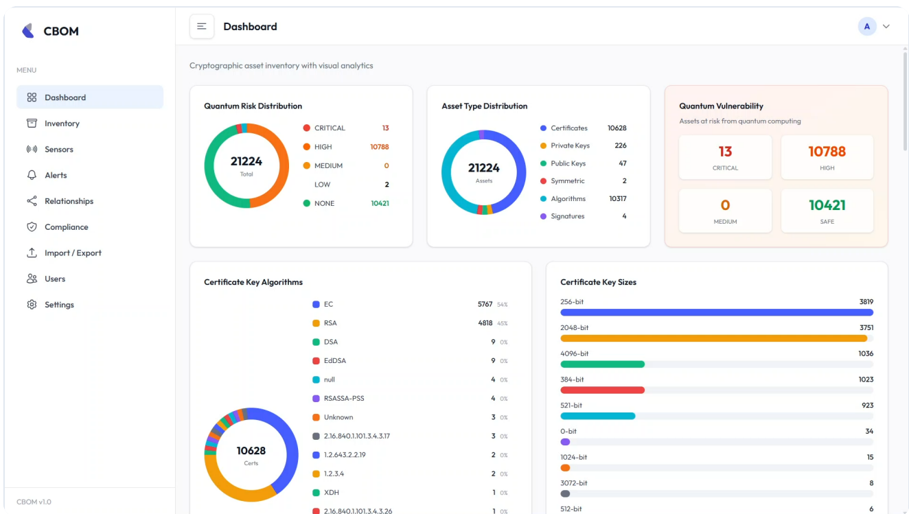
CBOM Discovery Dashboard — cryptographic asset inventory with quantum risk scoring, algorithm distribution, and compliance status.
